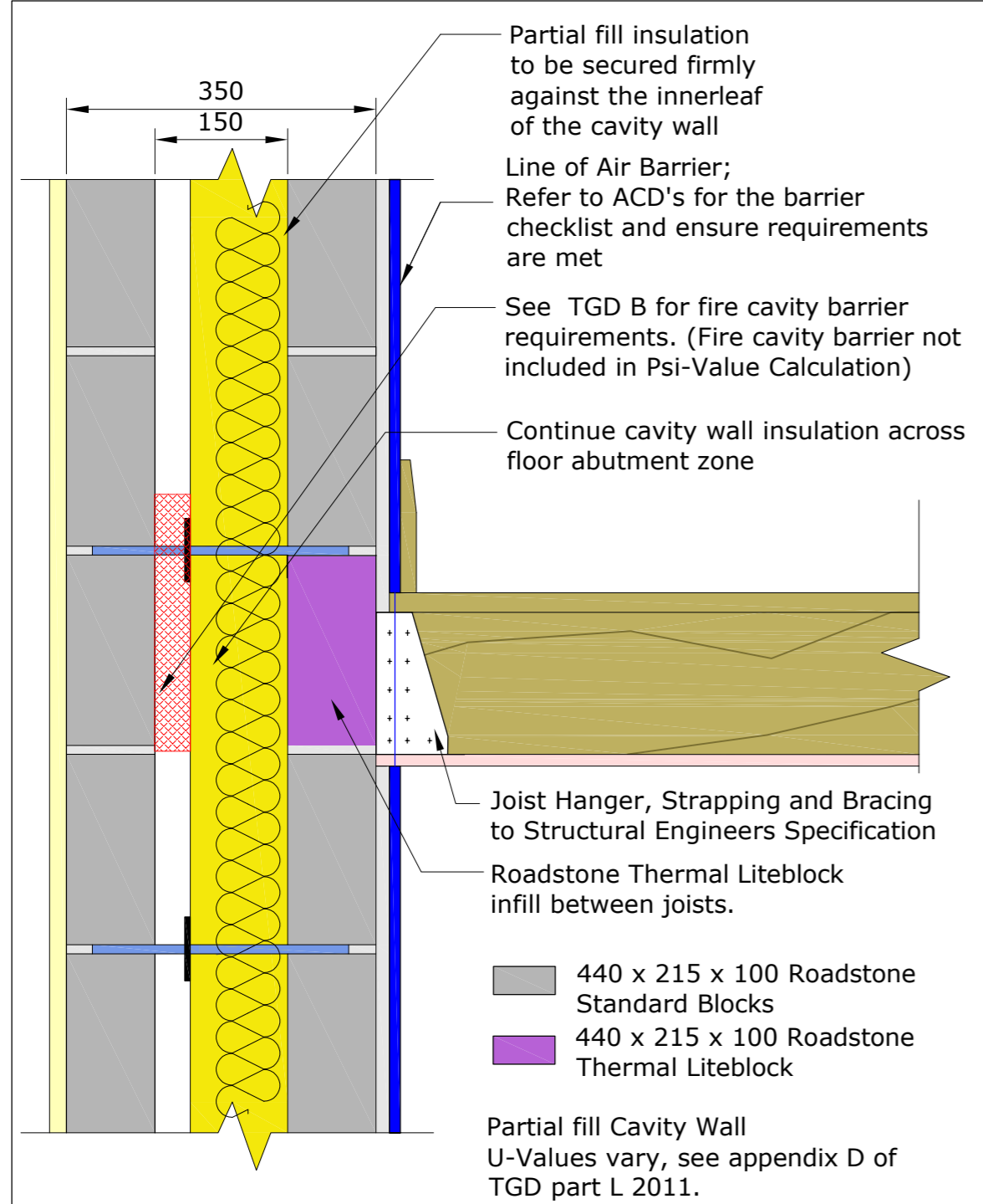
DETAIL RS1.05 JOISTS PERPENDICULAR
