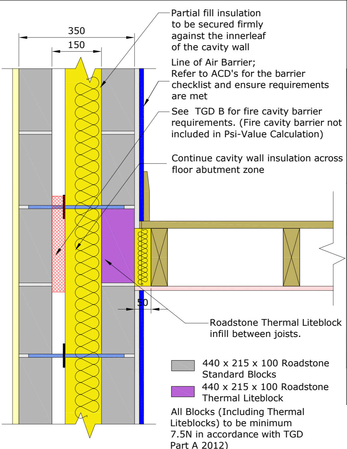
DETAIL RS1.05a JOISTS PARALLEL
