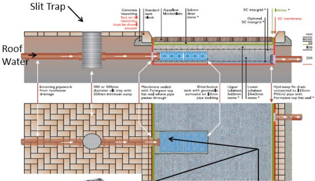
Distribution Tanks
