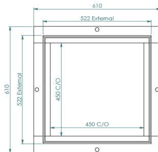
Recessed cross-section top view
