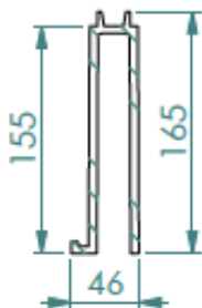
Modula cross-section detail
